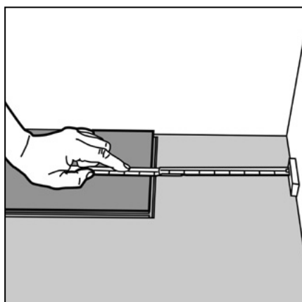
Figure 24 Last plank, first row
